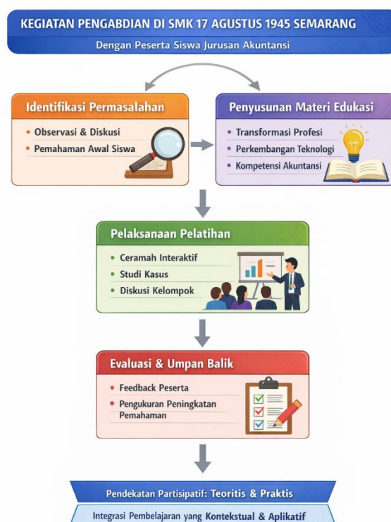
Gambar 1. Flowchart PKM
