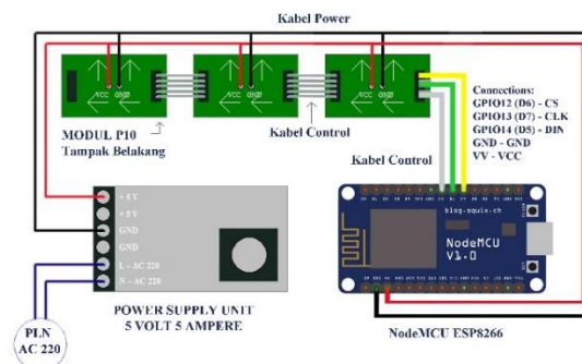
Gambar 4. Wiring Komponen Running Text LED
